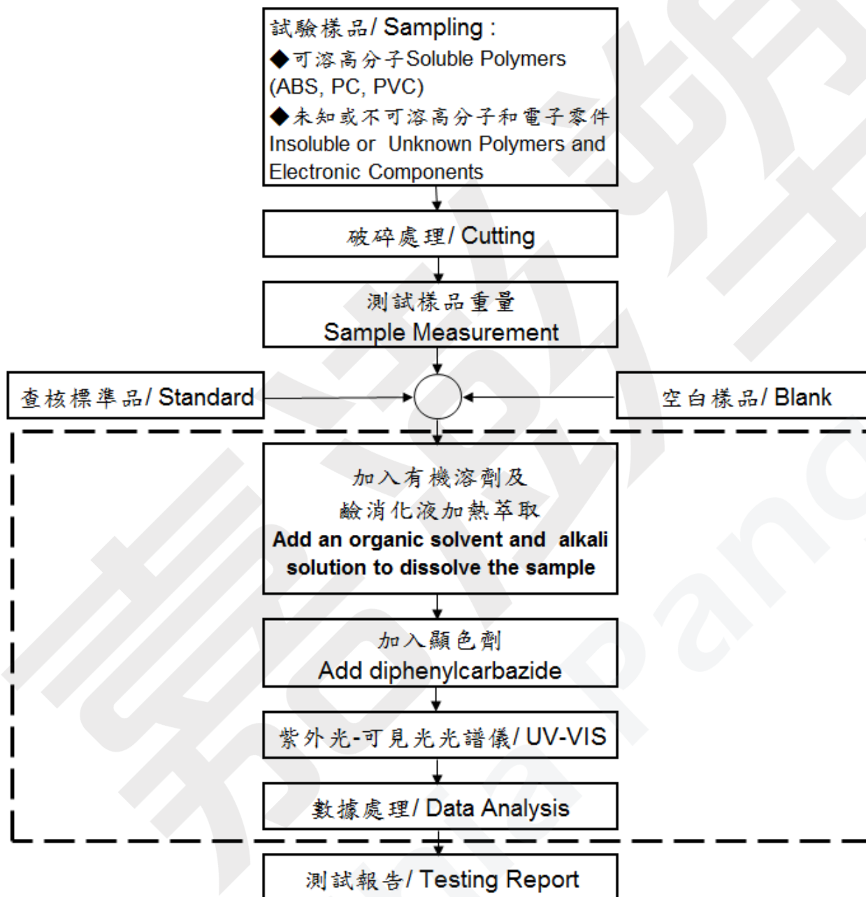
Flow Chart of Extraction-IEC 62321 for \text{Cr}^{6+}
